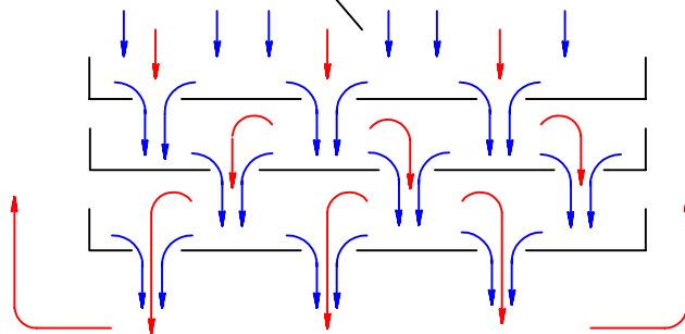
STEAM/WATER FLOW THROUGH CO-FLOW TRAYS
